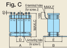
Filter dimensions (30kW or more);reactor
