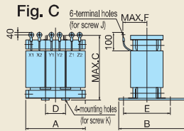
Filter dimensions (30kW or more);reactor
